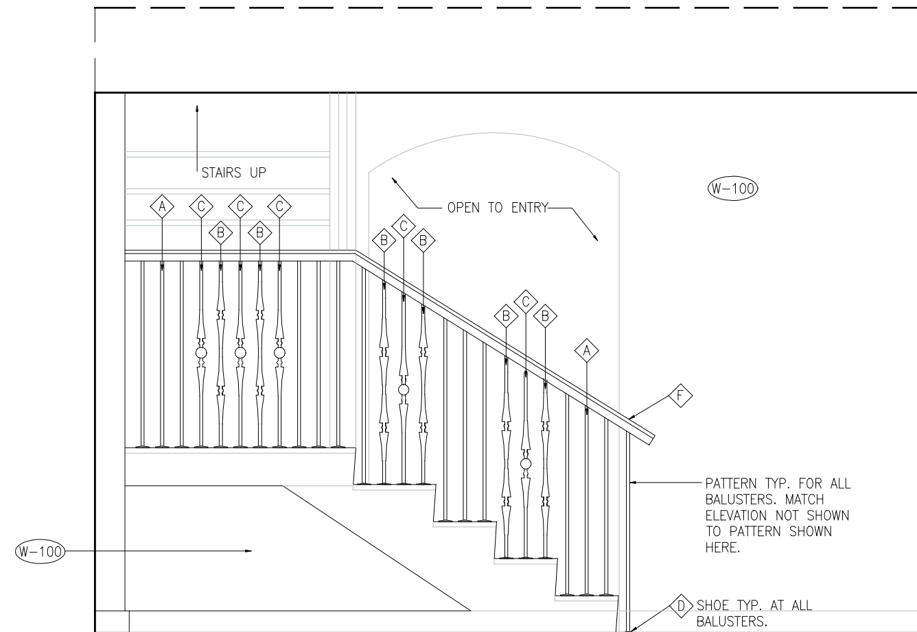
2 East Elevation - Stairs
