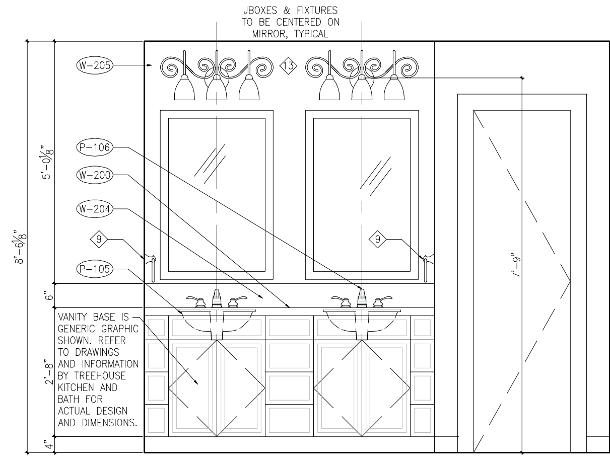
3 North Elevation - Master Bathroom SCALE: 1/2" = 1'-0"
