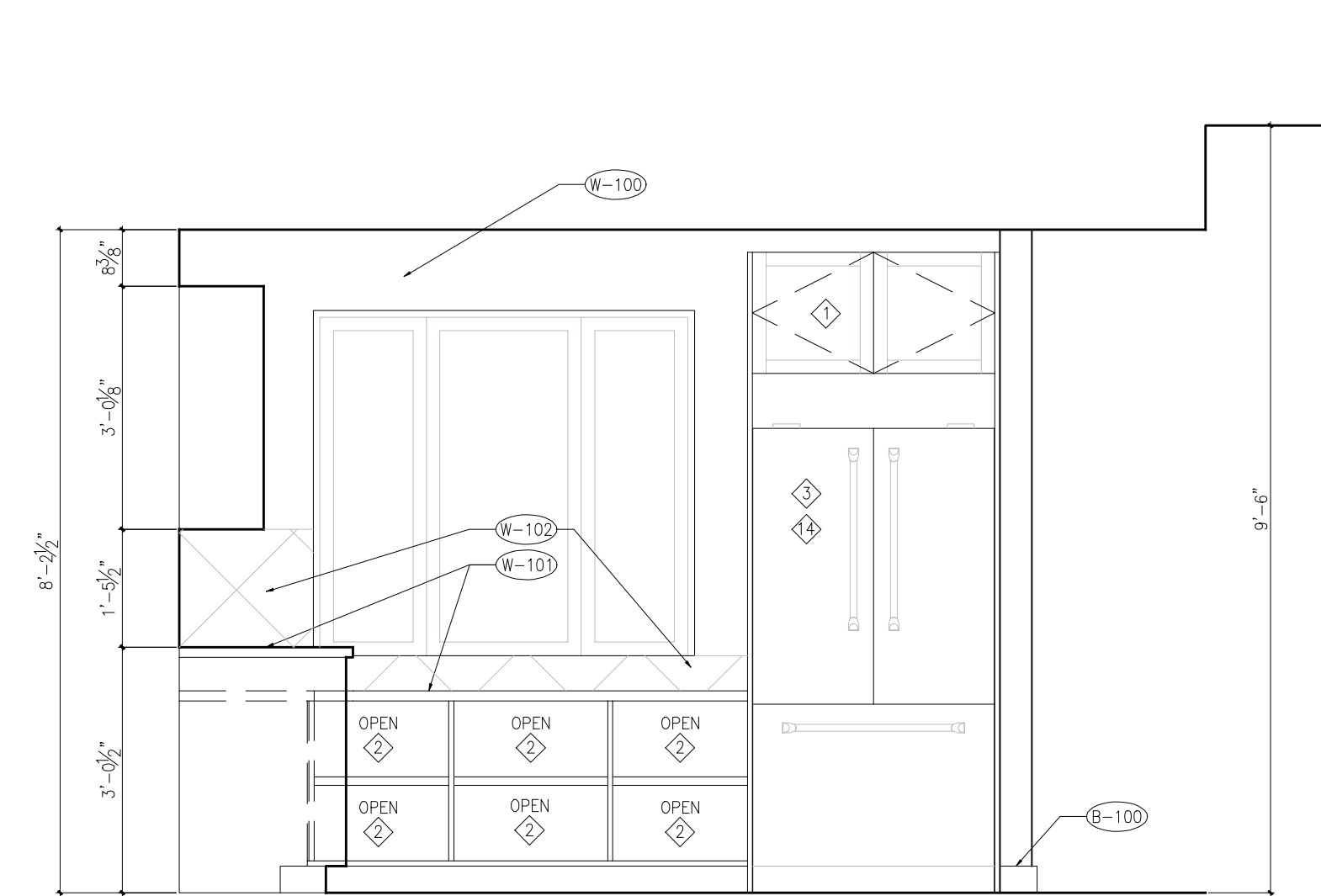
1 West Elevation - Kitchen
