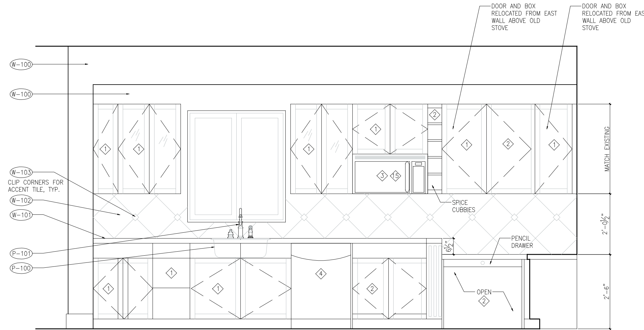
2 South Elevation - Kitchen
