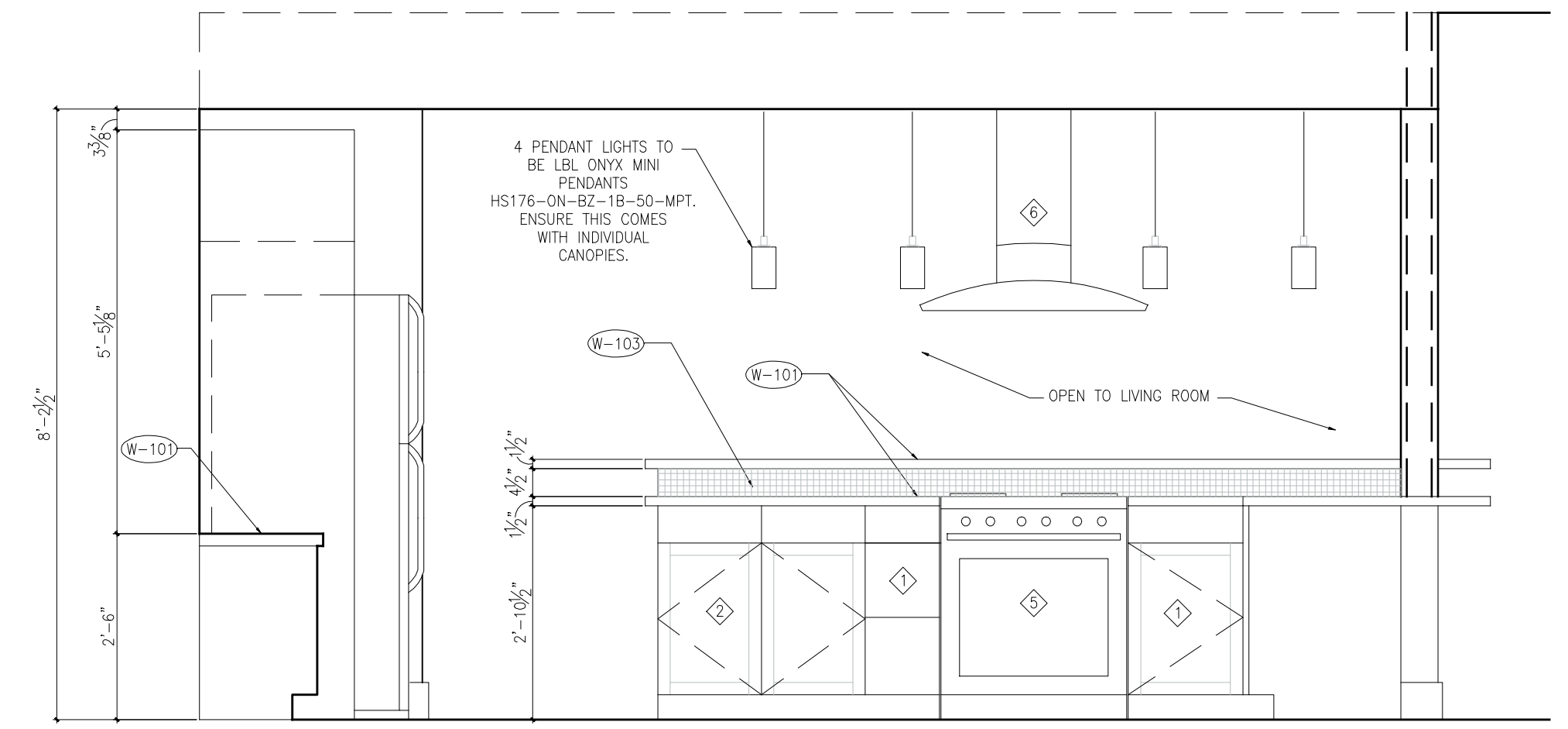
4 North Elevation - Kitchen
