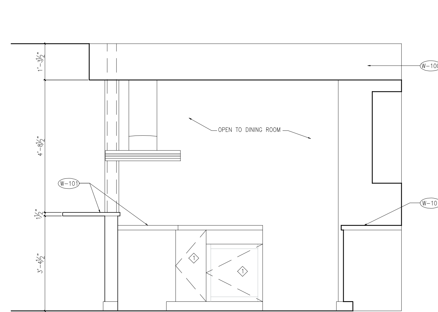
3 East Elevation - Kitchen
